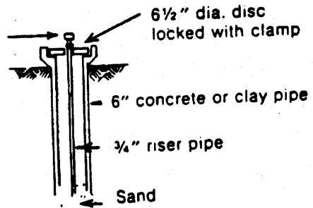
TYPE A DETAIL OF WATER RISER PIPE TYPE B DETAIL OF WATER RISER PIPE
